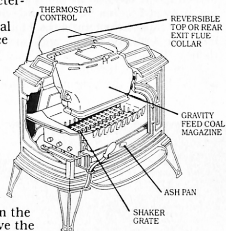
Detail of coal-burning Vigilant
