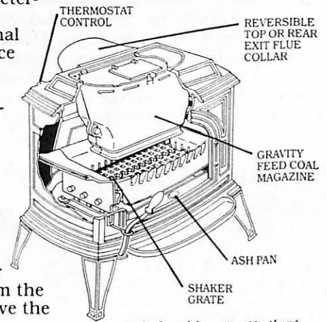
Detail of coal-burning Vigilant
