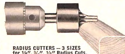
ADJUSTABLE BEVEL-CUTTER cuts 45° bevels from 1/32" to 3/16" wide.
