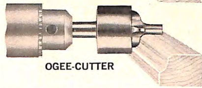
COVE-CUTTER
