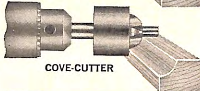
BEADING-CUTTER
