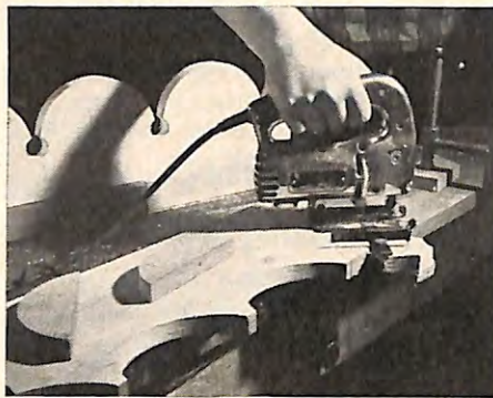
Make a cove-cut edge by swinging a saber saw on a nail driven into a block that is tacked into position against the edge for each circle cut. Scallops in rear were made by first boring 1" holes.
