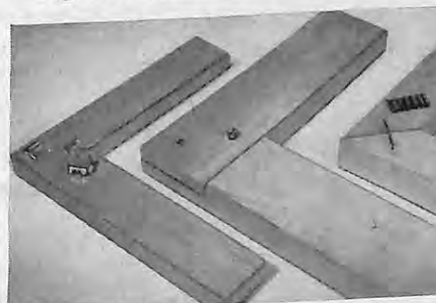
Typical corner joints. At left, a miter joint held with miter fasteners. Center, a half-lap secured with 1" wood screws. At right, miter joint with corrugated fasteners.
