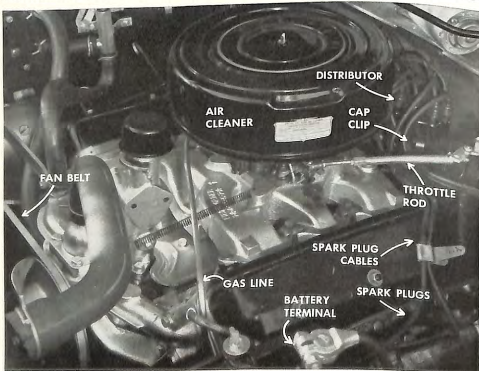
Spark plugs are set low, four to a side, in this V-8 engine. The ignition coil, not shown, can be found by following the center cable from the distributor head. In this car, the fuel filter is at the lower end of the gas line.
