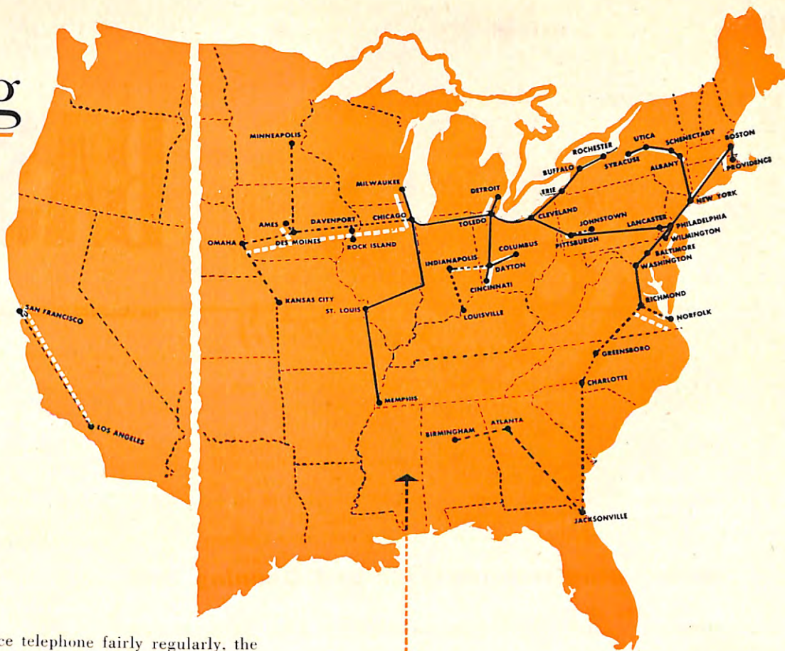
The television network today and the way it will be at the end of this year. Solid black lines show present coaxial cable routes; solid white lines show the present radio relay links. Dotted lines—black for coaxial; white for radio relay—indicate what's being added this year. In addition, radio relay links are under construction from New York to Chicago and New York to Washington, to supplement the present coaxial routes.
